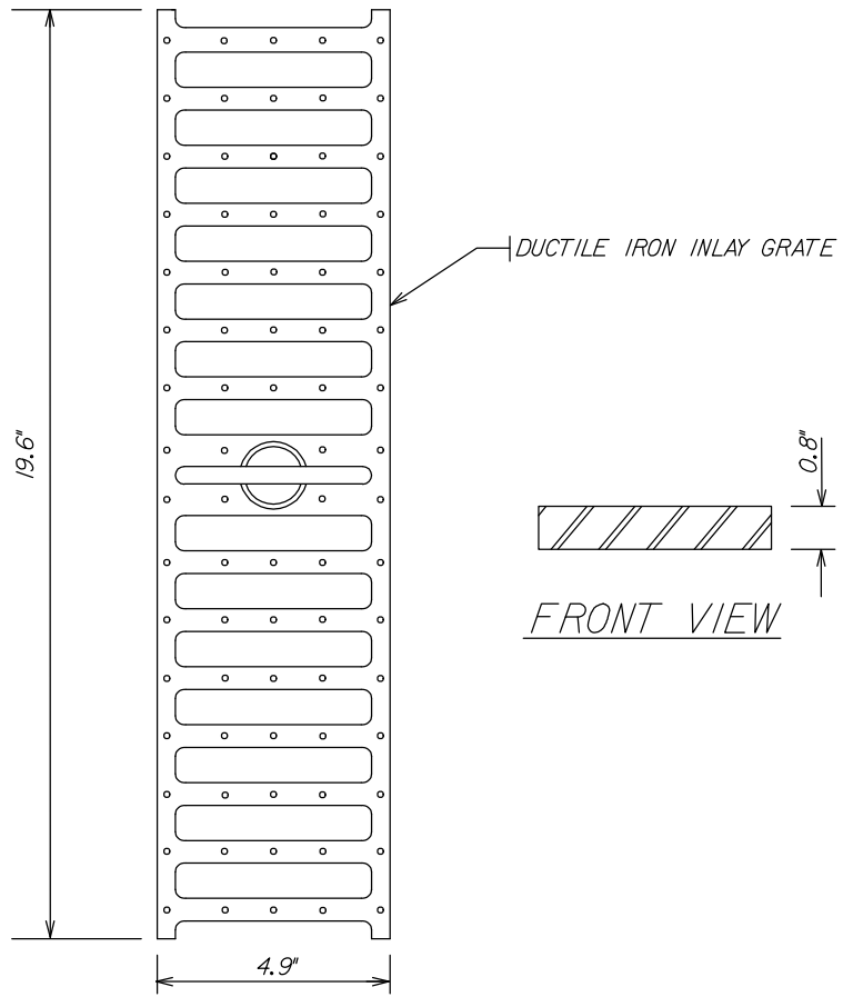
PLAN VIEW
