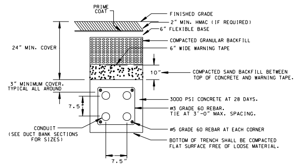
TYPICAL DUCT BANK SECTION N.T.S.
