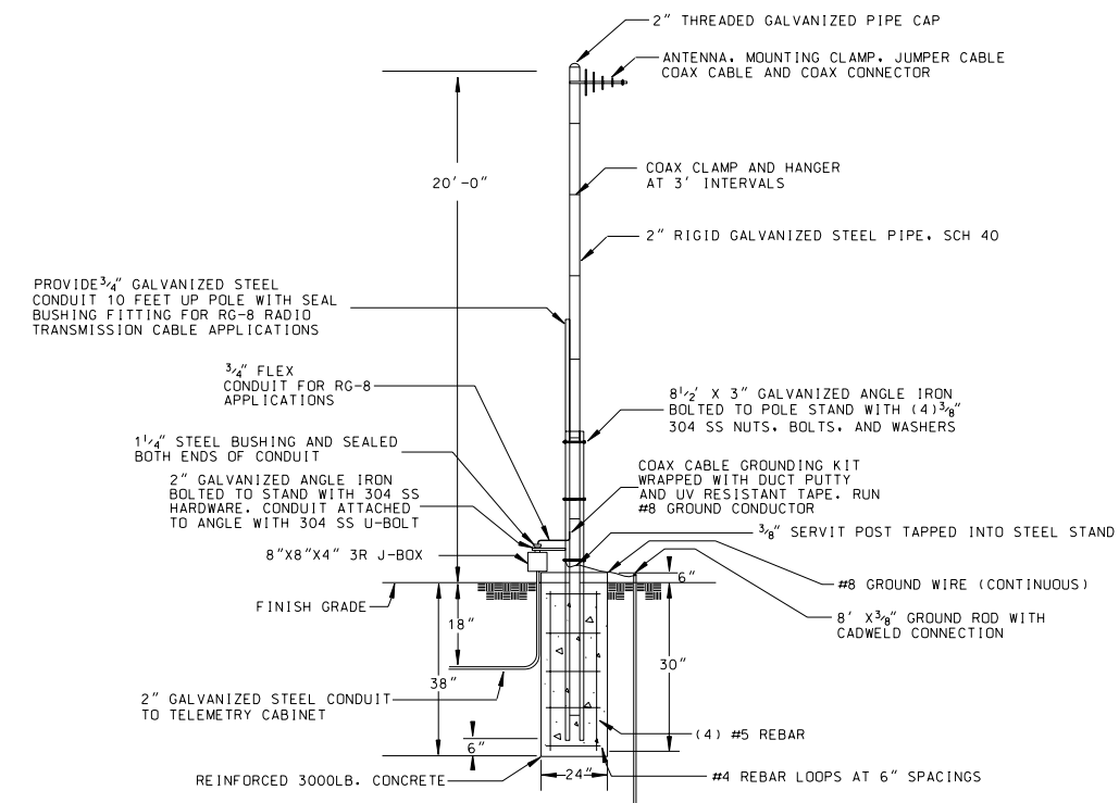
SIDE VIEW ANTENNA POST & FOUNDATION N.T.S.
