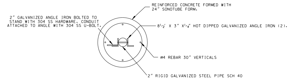
PLAN VIEW ANTENNA POST & FOUNDATION N.T.S.
