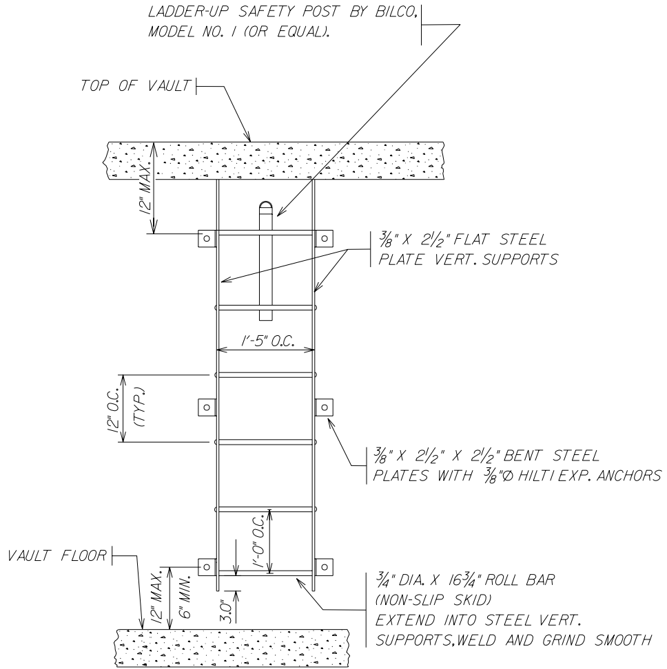
VAULT DETAIL
