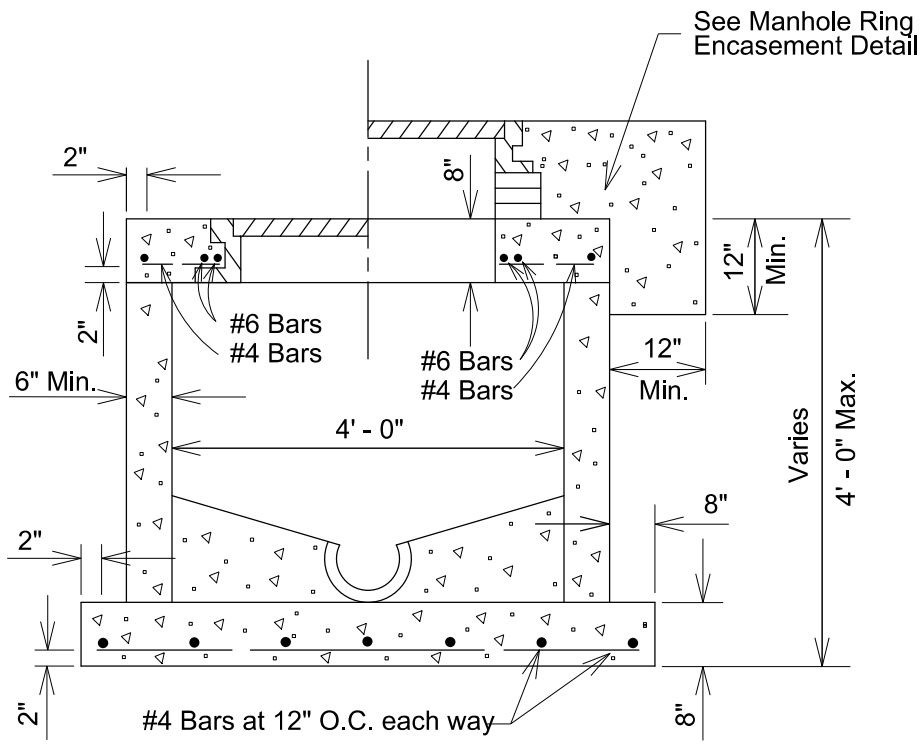
SHALLOW MANHOLE PRECAST OR MONOLITHIC
